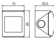
3联开关 3 Gang switch 13A-250V~ 表面安装 IP55 Surface mount
